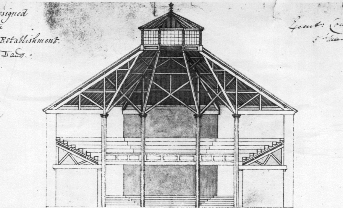
60 feet. Transverse Section.
